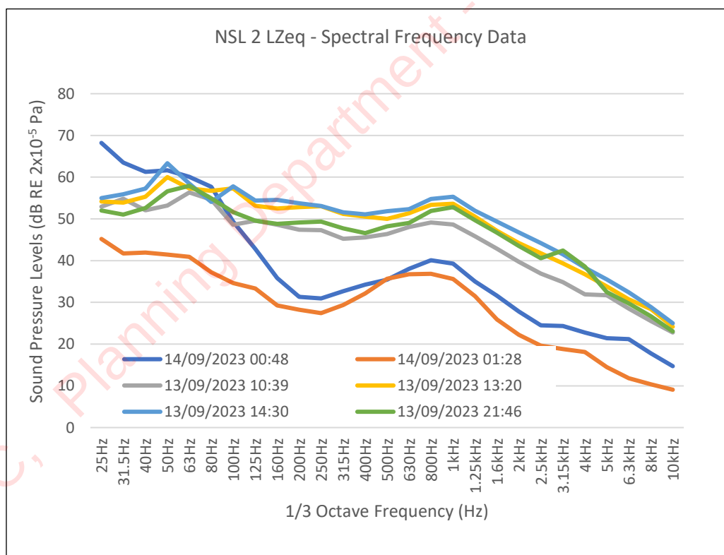
Figure B2 NSL 2 – 1/3 rd Octave Band Spectrum for Night Survey
