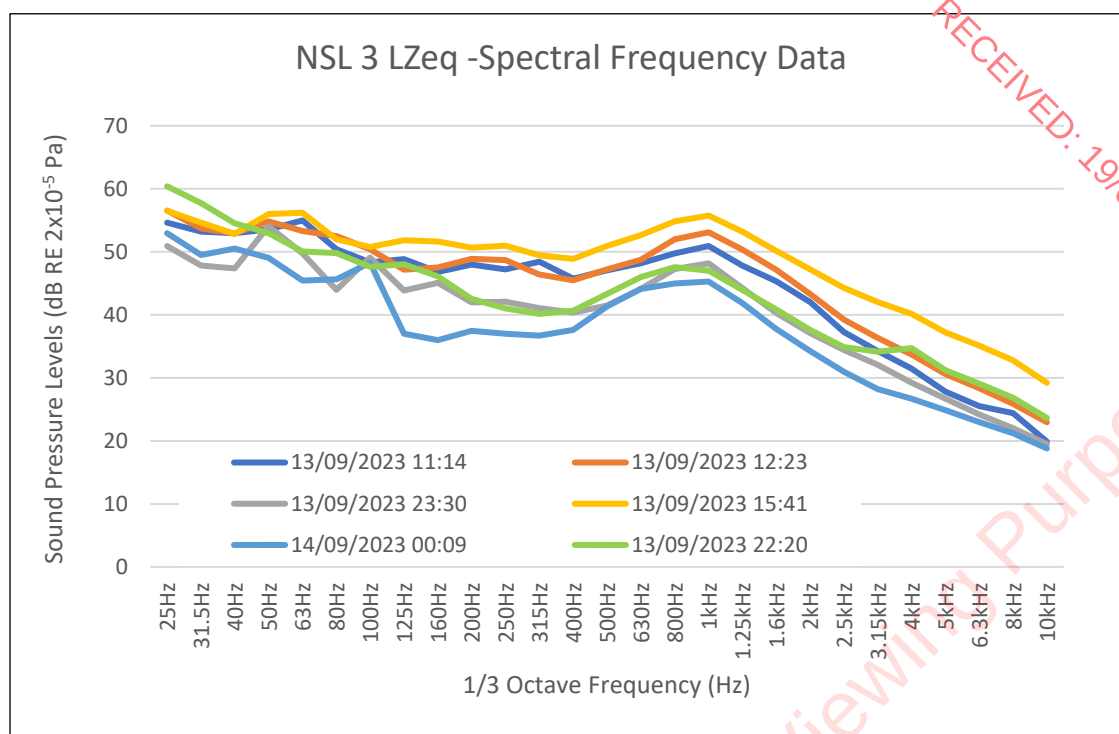
Figure B3 NSL 3 – 1/3 rd Octave Band Spectrum for Night Survey
